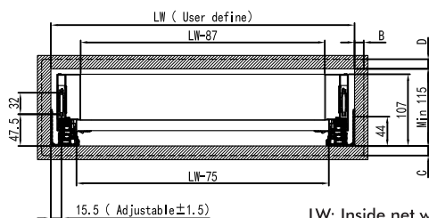
Space required
