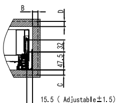
Front panel dimensions
