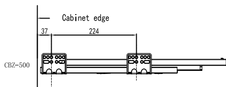
Installation dimensions for cabinet rail
